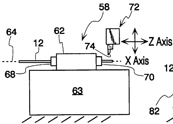
Fig. 12 (PRIOR ART)
