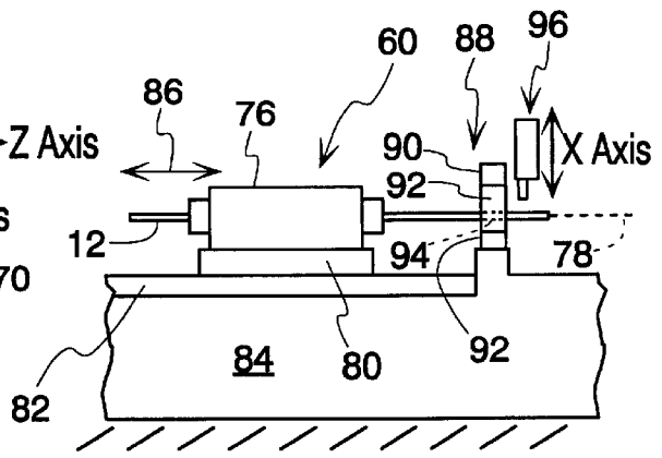
Fig. 13 (PRIOR ART)
