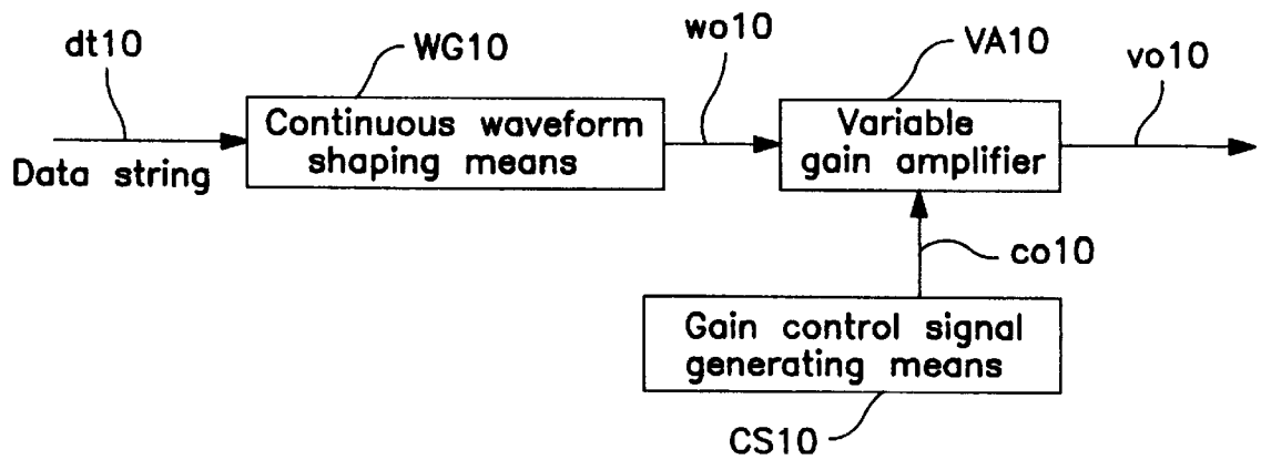
FIG. 11 PRIOR ART
