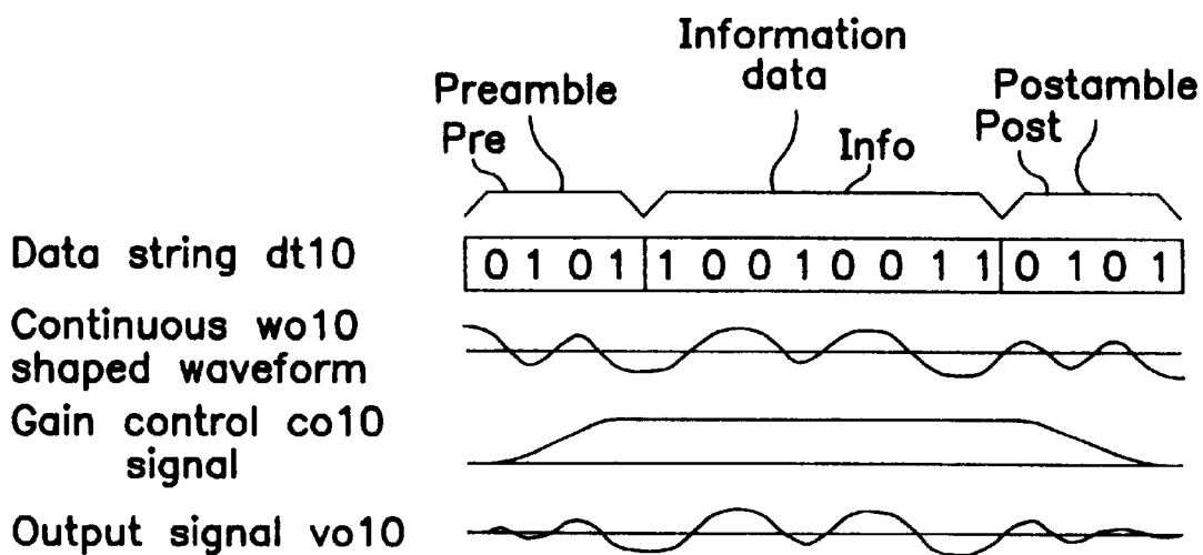
FIG. 12 PRIOR ART
