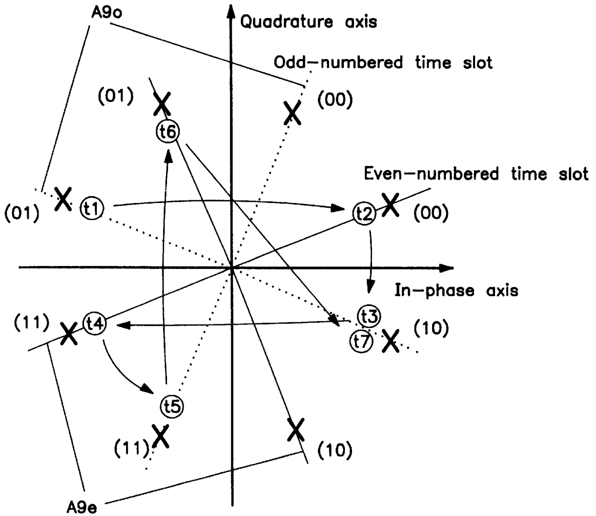
FIG. 10 PRIOR ART
