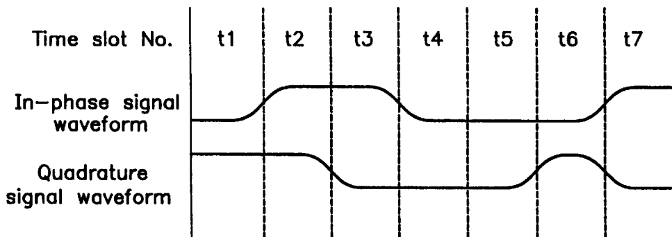
FIG. 5C PRIOR ART
