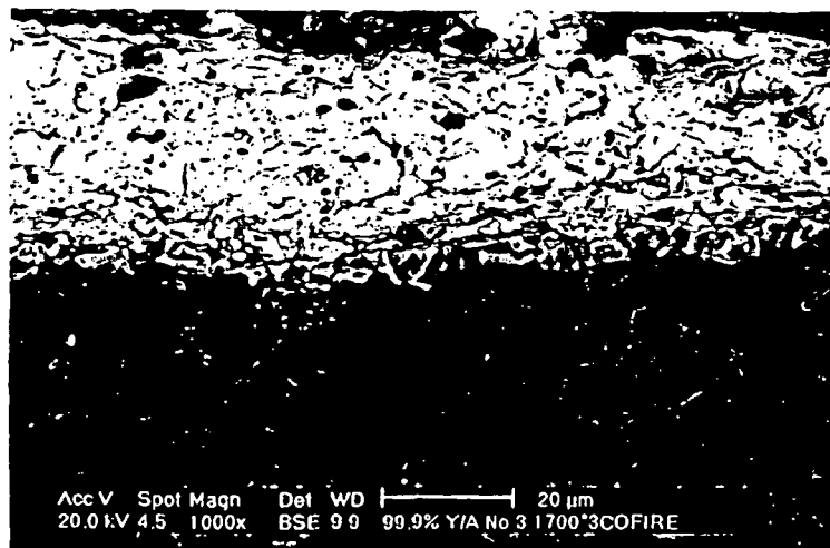
Surface of 1700°C Co-sintered product (X1000)
