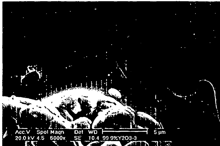
Surface of 99.9% Y_2O_3 sprayed product ( \times 5000 )
