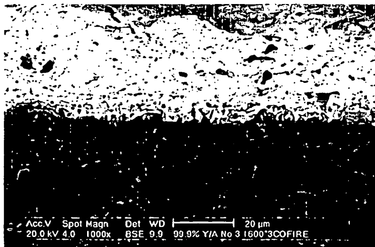
Surface of 1600°C Co-sintered product (×1000)
