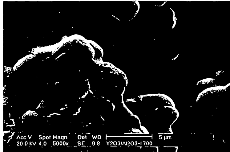
Surface of 1700°C X 3h Co-sintered product (X5000)
