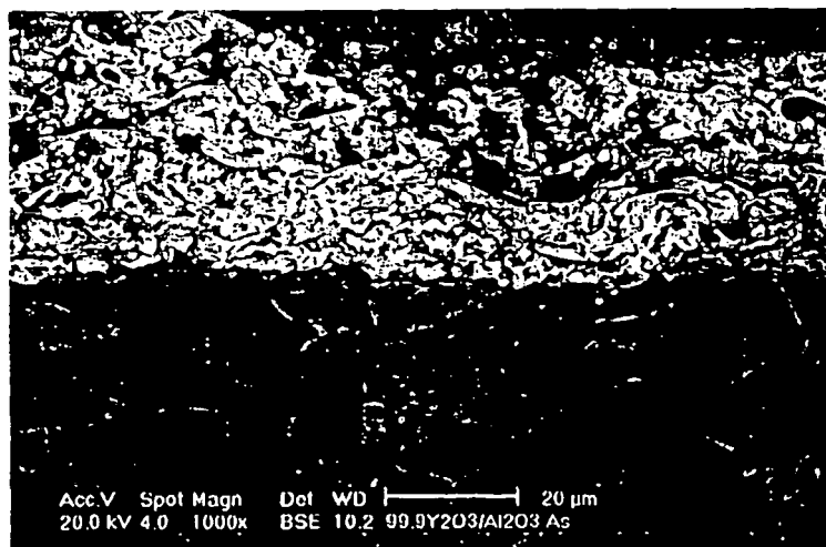
Section of 99.9% Y_2O_3 sprayed product ( \times 1000 )
