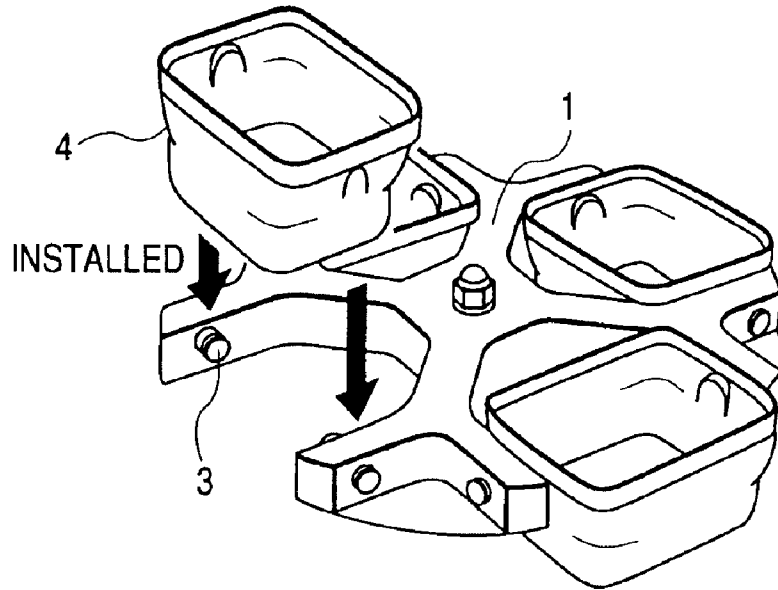
FIG. 8 PRIOR ART
