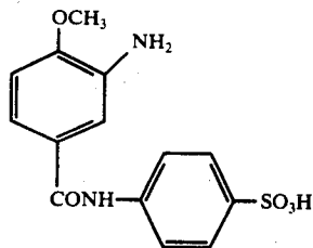
7. The compound of the formula
