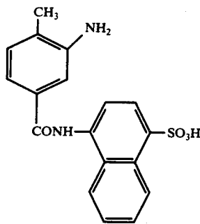
7. The compound of the formula
