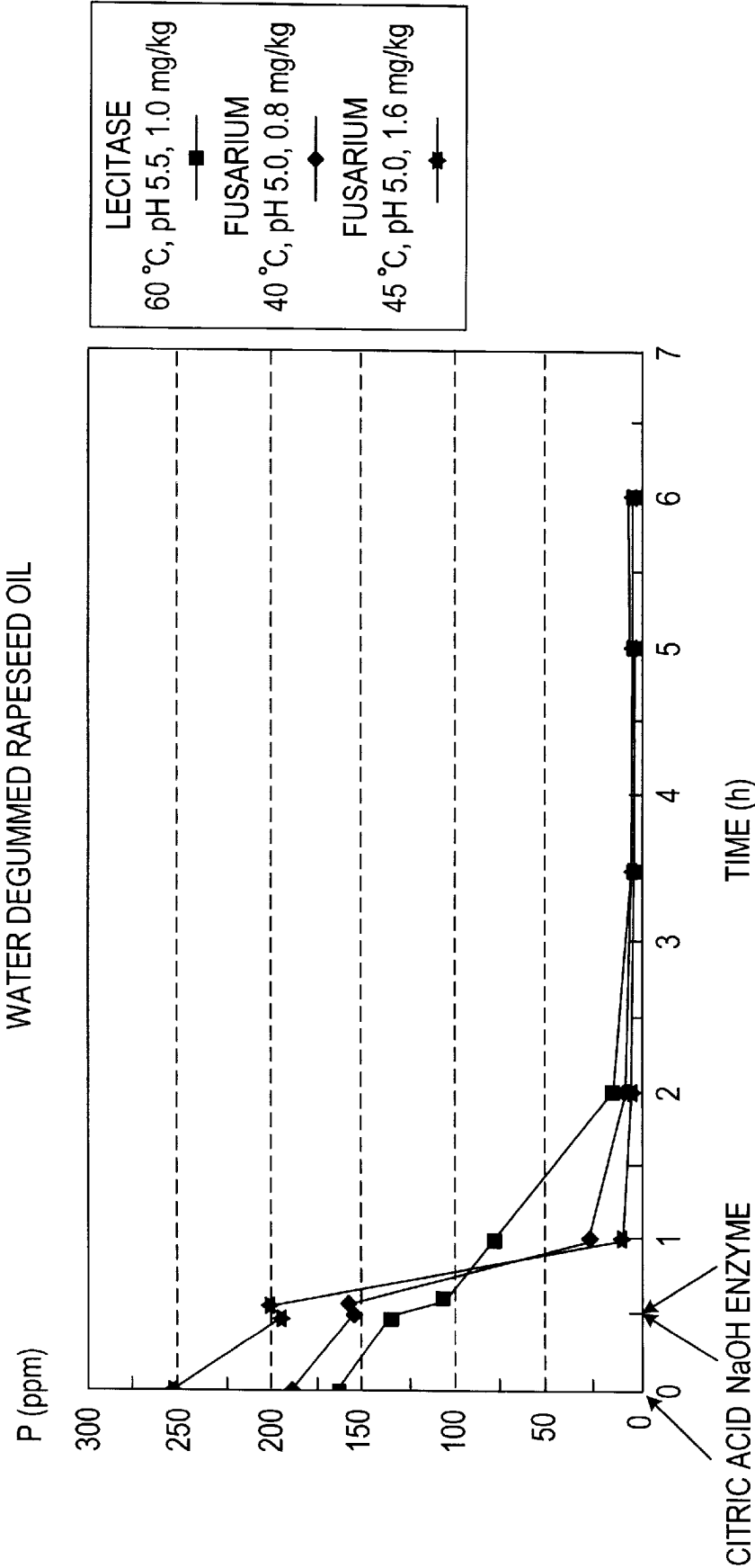
FIG. 2 OIL DEGUMMING - FUSARIUM PL VS. LECITASE
