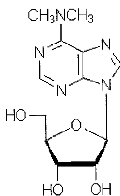
N6,N6-dimethyladenosine
