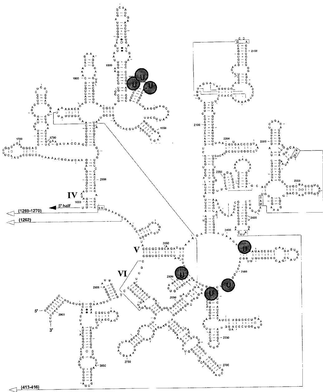
Figure 14 Uridine (grey) residues in 23S rRNA that are substrates for a pseudouridine synthase.
