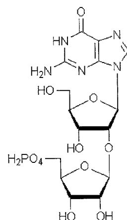
2'-O-ribosylguanosine (phosphate)
