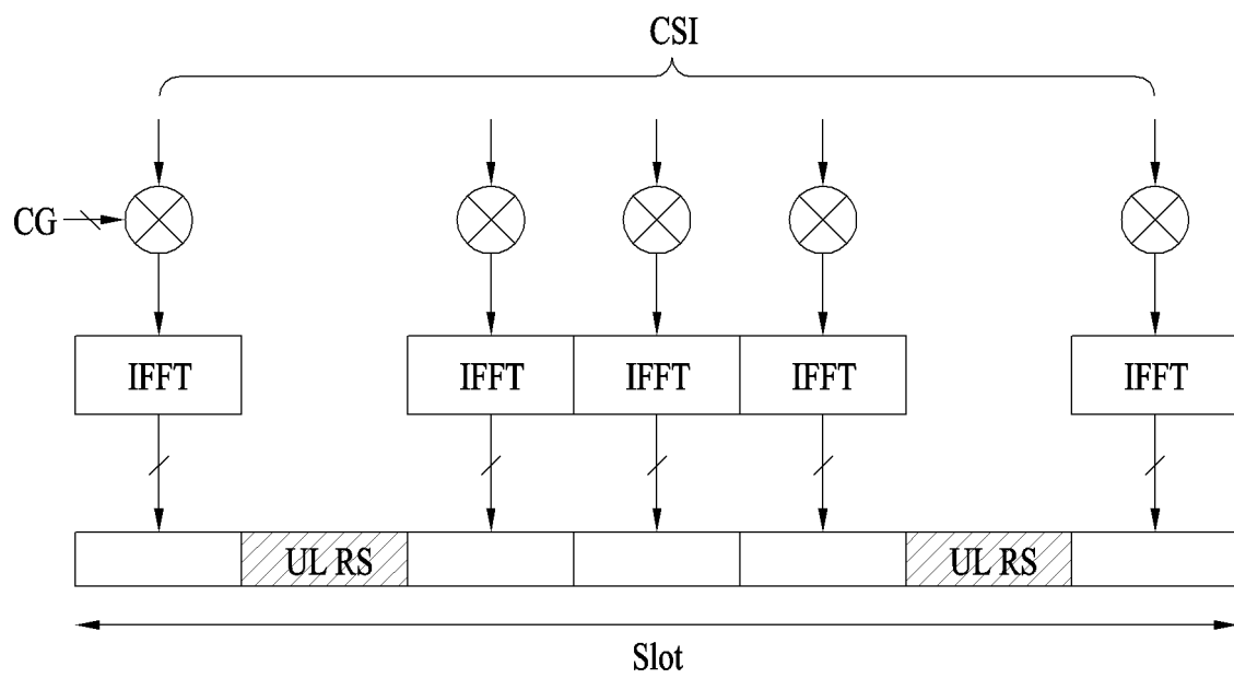
PUCCH format 2/2a/2b structure (normal CP)
