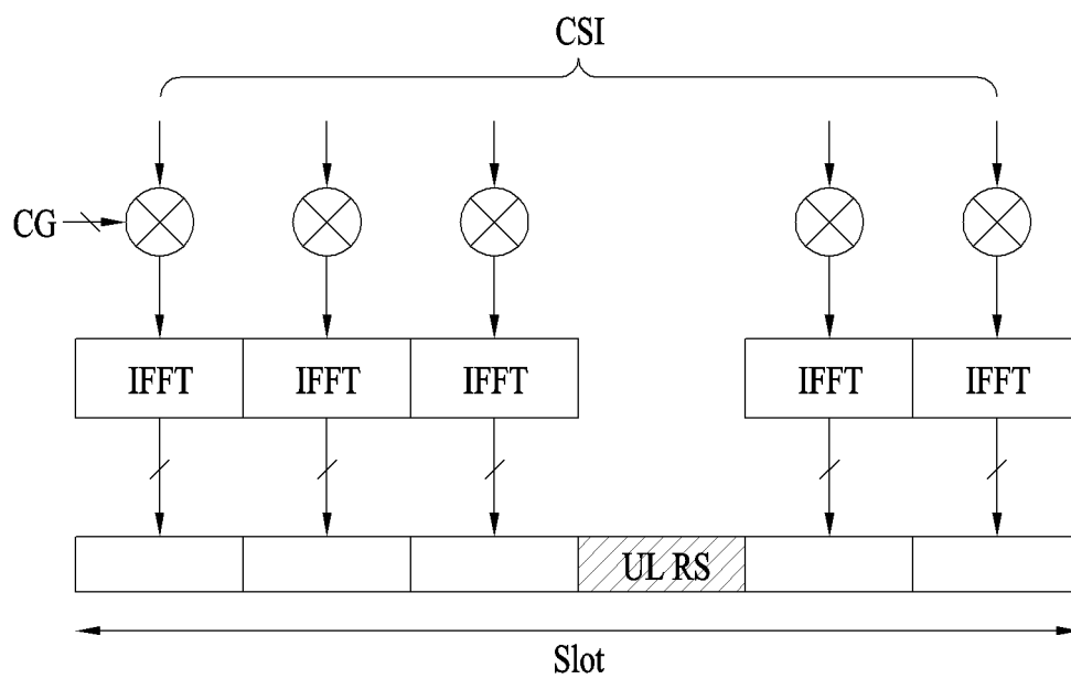
PUCCH format 2/2a/2b structure (extended CP)
