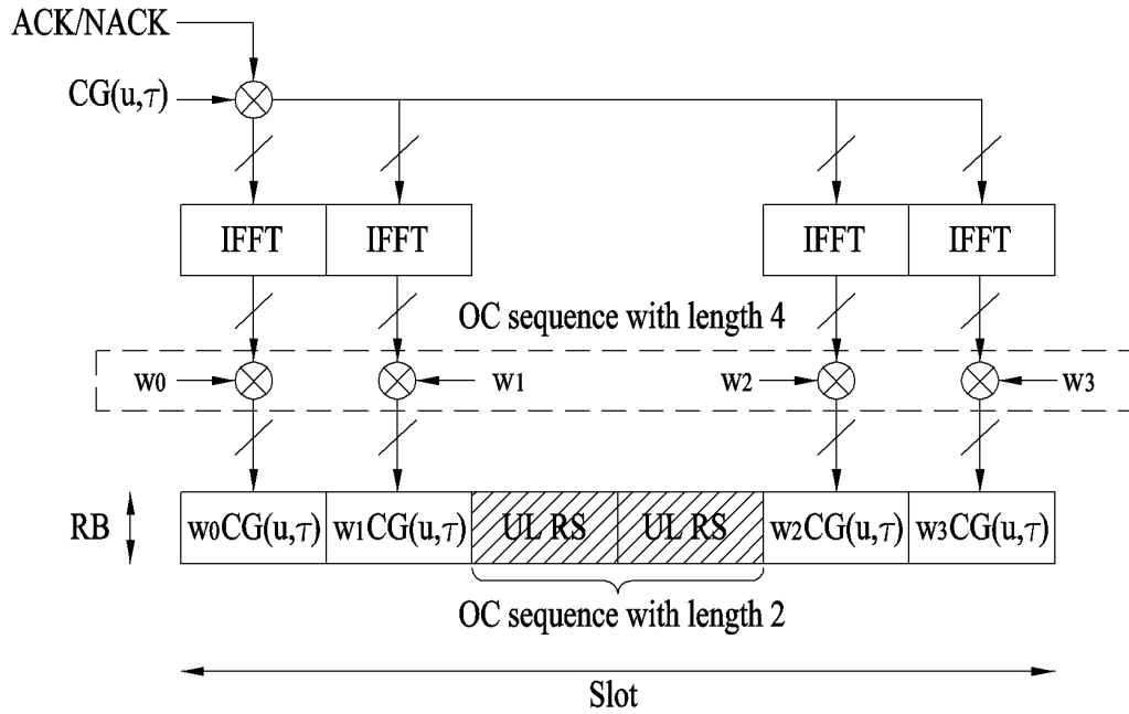
PUCCH format 1a/1b structure (extended CP)
