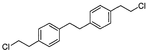
Step B 1-{2-[(2-Chloro-ethyl)-benzene]-ethyl}-4-(2-chloro-ethyl)-benzene
