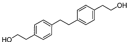
Step A 2-(4-{2-[4-(2-Hydroxy-ethyl)-phenyl]-ethyl}-phenyl)-ethanol
