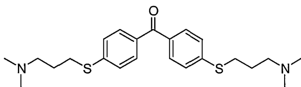
Bis-[4-(3-dimethylamino-propylsulfanyl)-phenyl]-methanone dihydrochloride K_i = 14 nM
