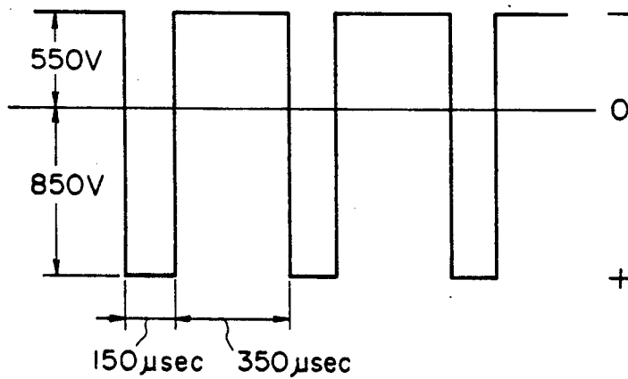
WAVEFORM OF SUPPLY 9
