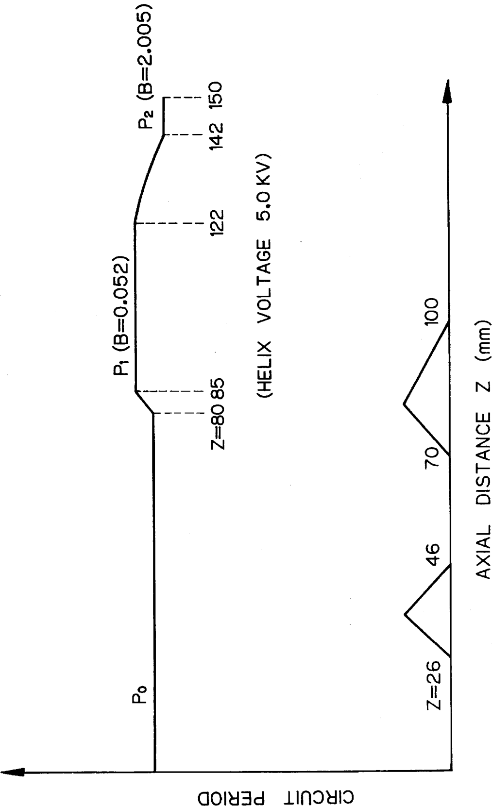
Fig. 6 PRIOR ART
