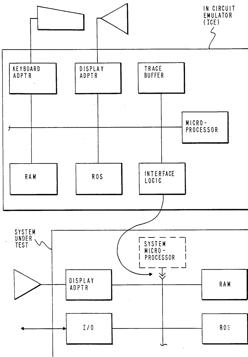
FIG. 1 PRIOR ART
