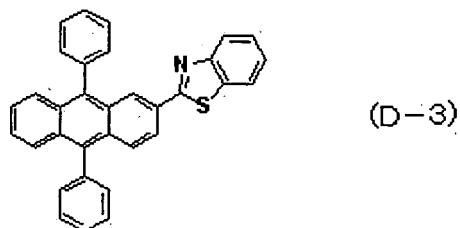
[Chemical formula 26]
