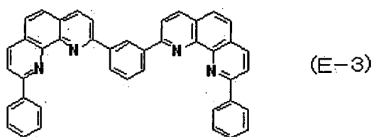
[Chemical formula 28]
