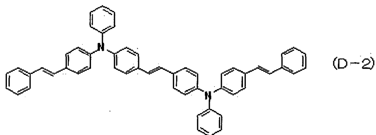
[Chemical formula 25]
