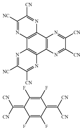
F4-TCNQ
