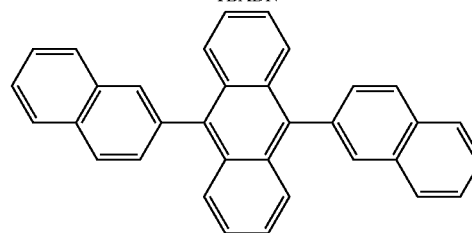
TBADN
