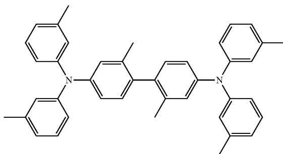
HMTDP
