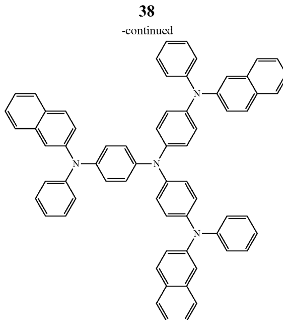
2-TNATA
