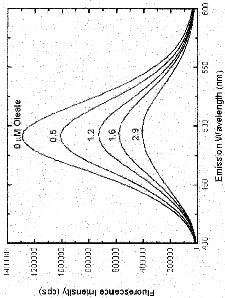
Fluorescence emission spectra for ADIFAB K27C during titration with sodium oleate at 22°C. Ex = 386nm
