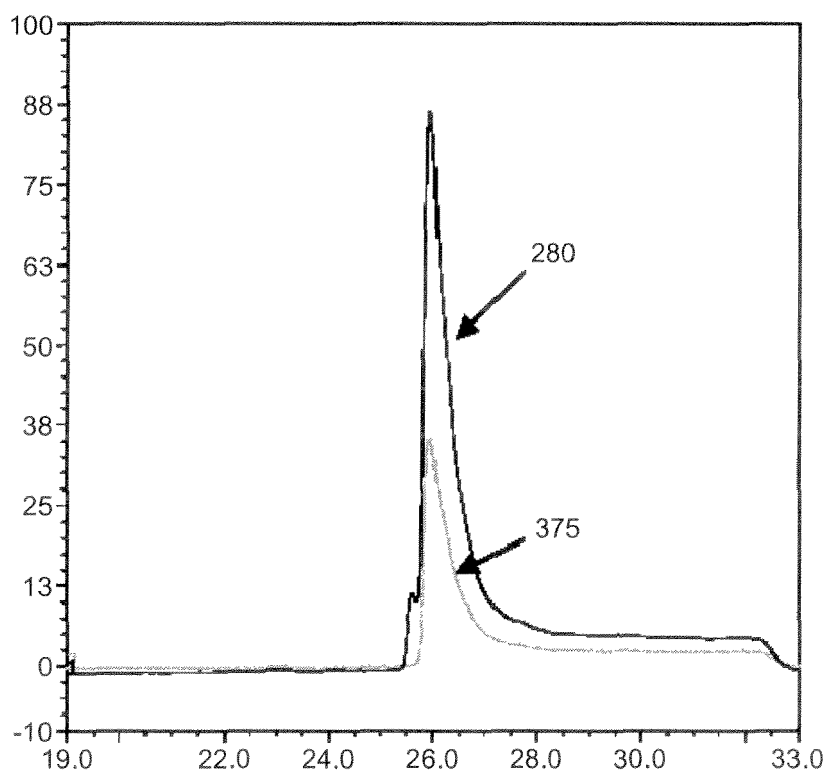
HPLC trace of ADIFAB. The 280 nm and 375 nm traces correspond to the protein and acrylodan respectively
