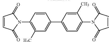
1,1'-(3,3'-dimethyl-1,1'-biphenyl-4,4'-diyl) bismaleimide
