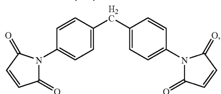
1,1'-(methylenedi-4,1-phenylene) bismaleimide
