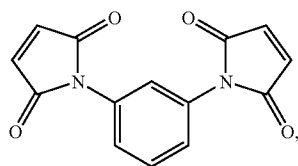
m-phenylene dimaleimide
