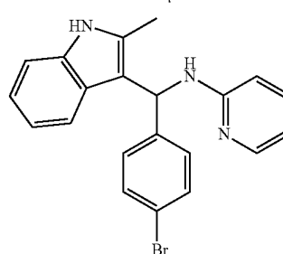
15: 17.2 \mu M
