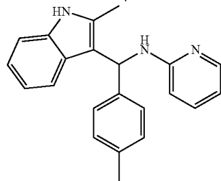
11: 9.5 \mu M
