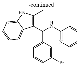
14: 14.1 \mu M
