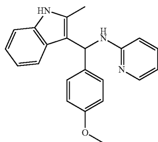
11: 9.5 \mu M
