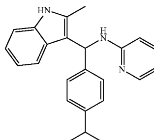
17: 15.3 \mu M
