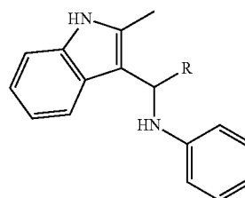
Scheme 2.
