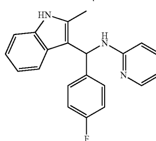
16: 28.9 \mu M
