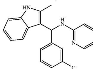
18: 25.1 \mu M
