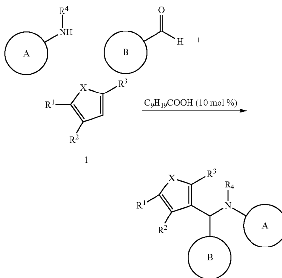
Scheme 1. Exemplary Synthesis
