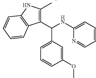
13: 30.3 \mu M
