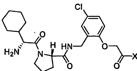
Scheme 1.5 Chemical structure corresponding to the building block combination X-REA001710-REA001712-BBA000031
