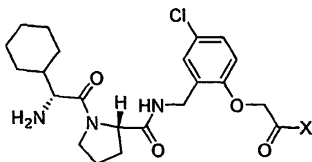
Scheme 2.4 Chemical structure corresponding to the building block combination X-REA001710-BBA001023-BBA000031
