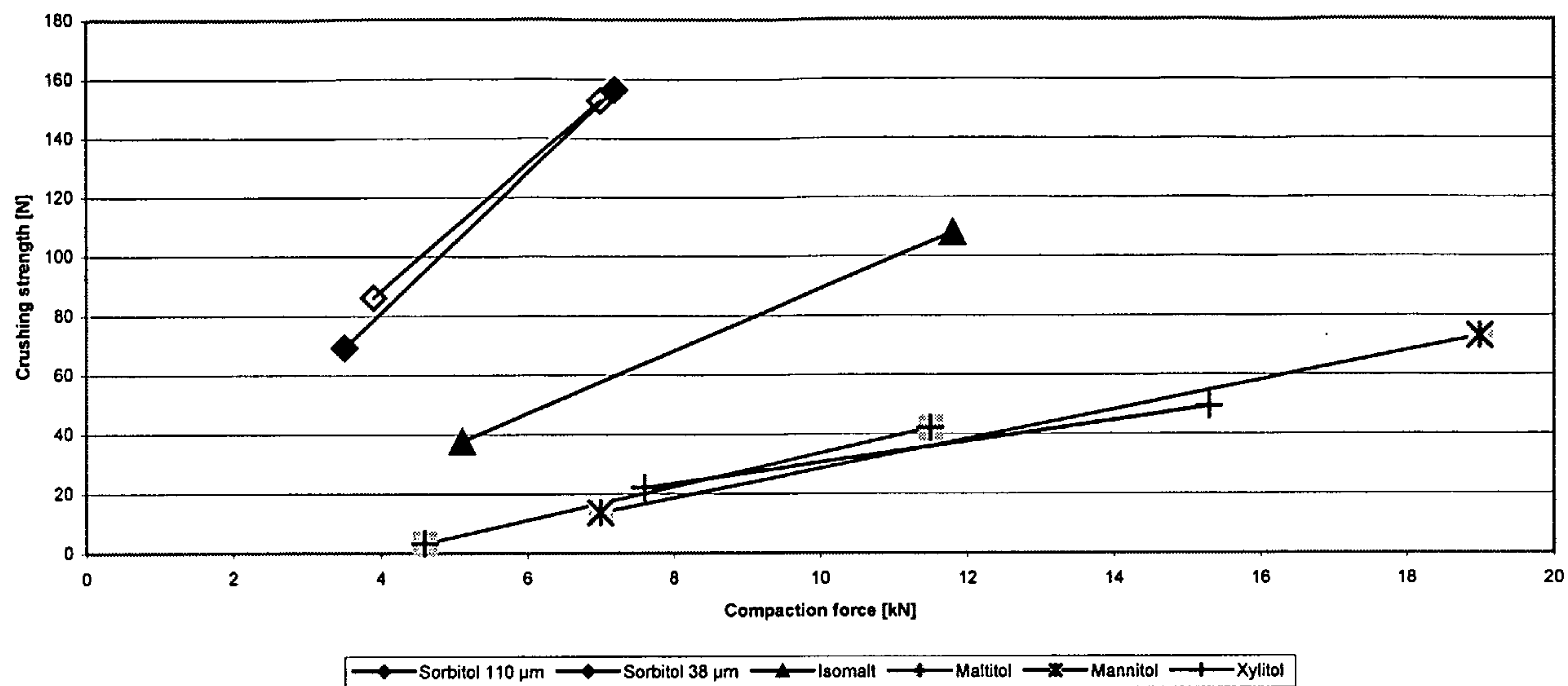
Compaction properties of sugar alcohols
