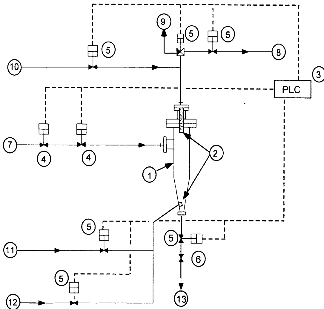
Figure 1. Automated Sampling System
