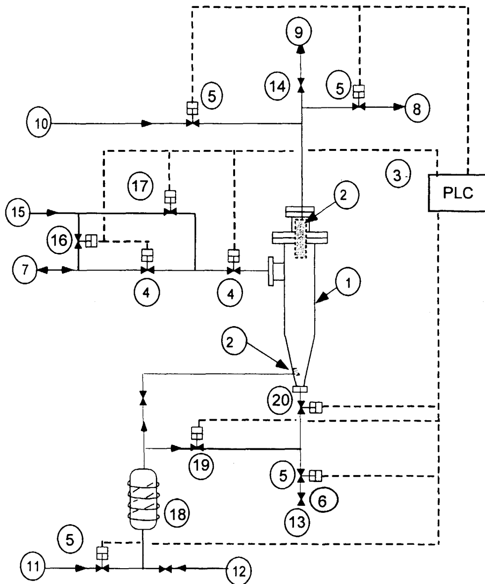
Figure 2. EPR-1 Commercial Reactor Sampling System
