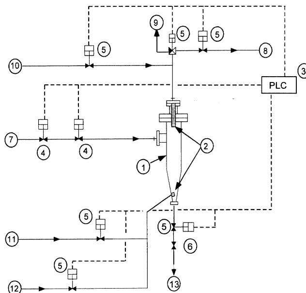
Figure 1. Automated Sampling System
