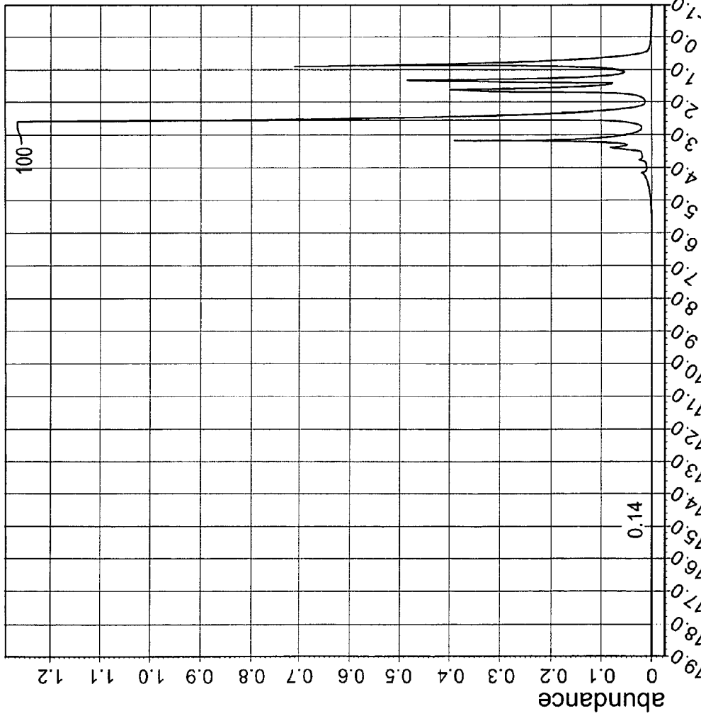
FIG. 6A X : parts per Million : 1H
