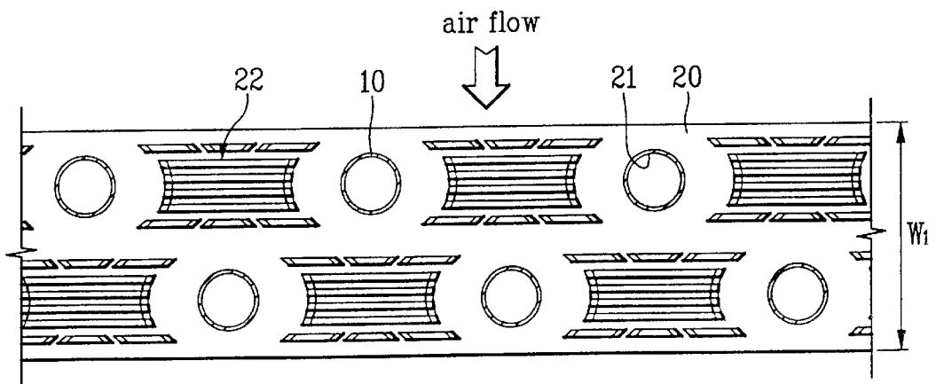
FIG.2 Prior Art
