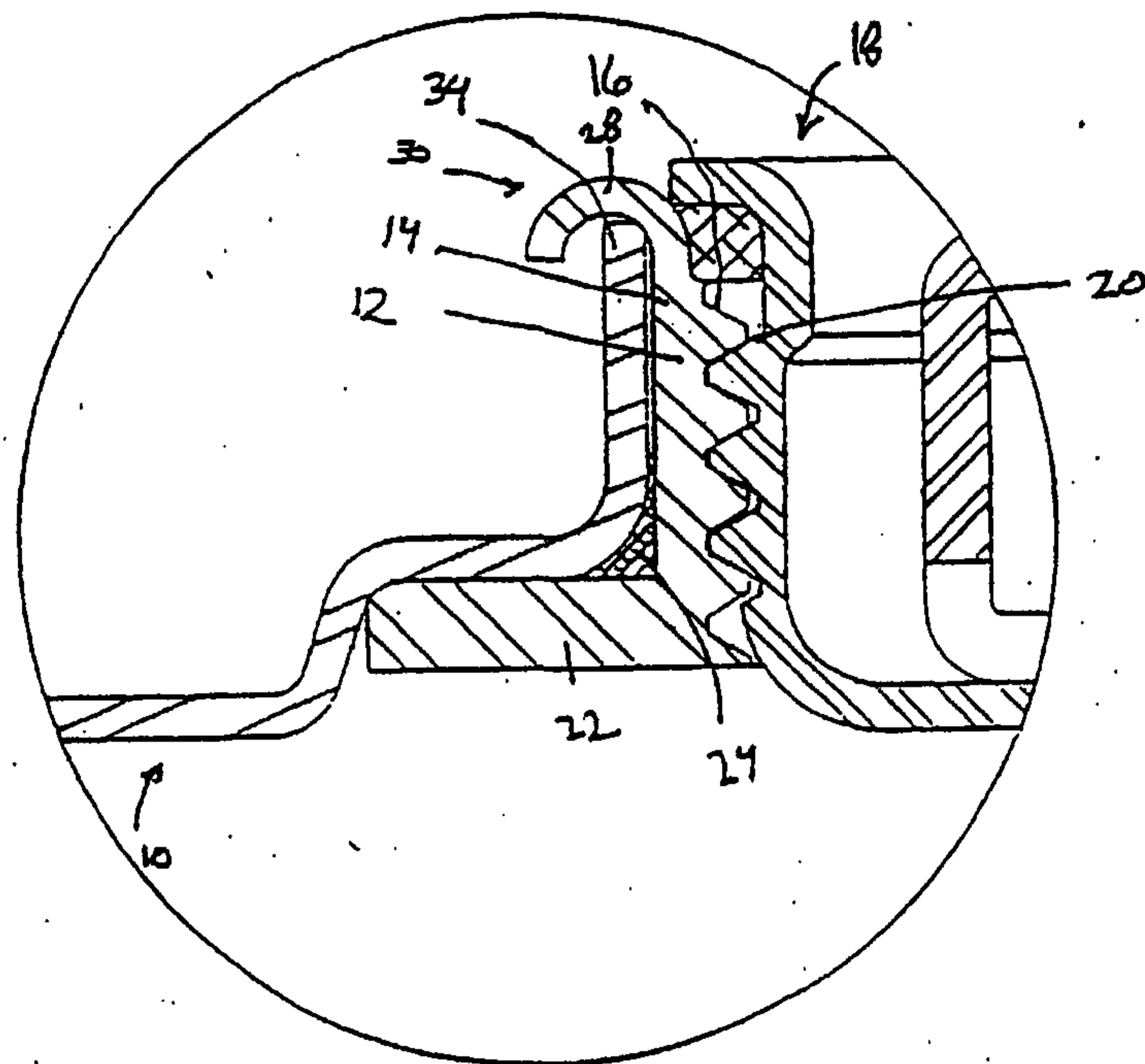
FIG. 2 PRIOR ART
