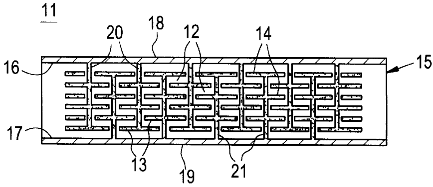
FIG. 9 PRIOR ART
