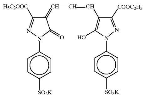
Compound (15)
