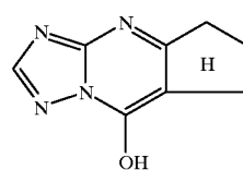
Sensitizing dye (1)
