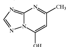
Compound (I-3)
