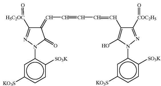
Compound (13)
