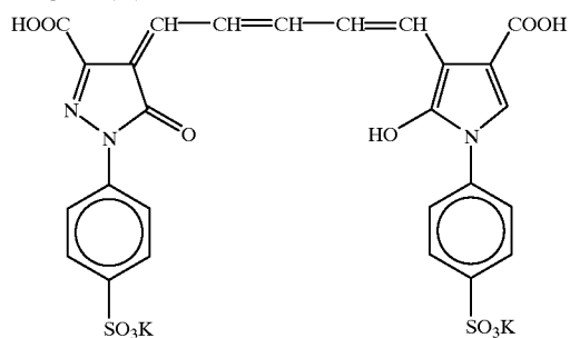
Compound (16)
