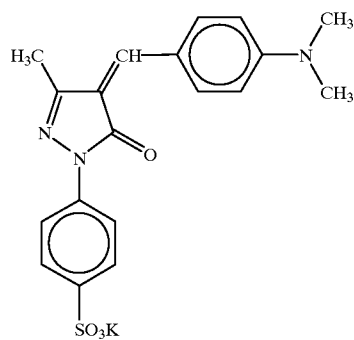
Compound (14)
