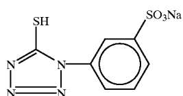
Compound (1)
