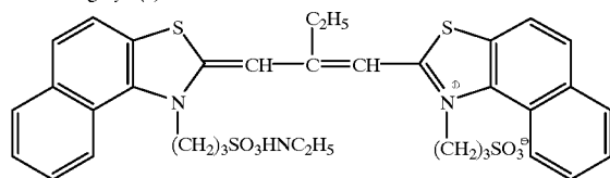
Sensitizing dye (4)
