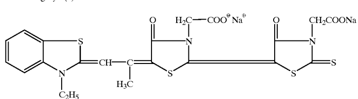
Sensitizing dye (5)
