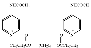
Compound (12)
