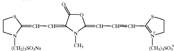
Sensitizing dye (5)
