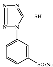
Compound (I-2)
