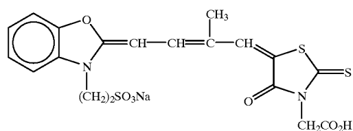
Compound (1)
