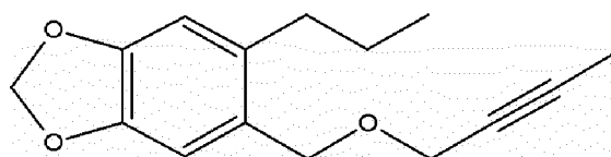
5-(but-2-ynyloxymethyl)-6-propyl-benzo[1,3]dioxole
