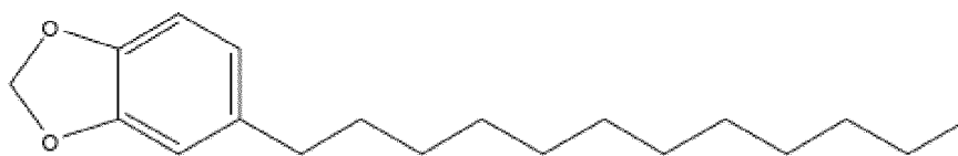
5-dodecylbenzo[d][1,3]dioxole (Formula XVI)
