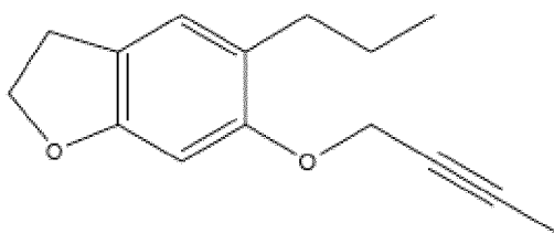
6-(but-2-ynoxy)-5-propyl-2,3-dihydrobenzofuran (Formula XVII)
