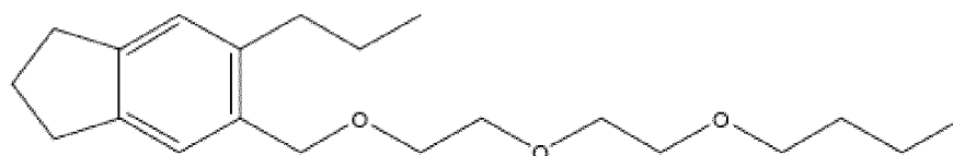
5-((2-(2-butoxyethoxy)ethoxy)methyl)-6-propyl-2,3-dihydro-1H-indene (Formula XIX)
