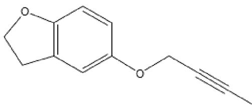
5-(but-2-ynoxy)-2,3-dihydrobenzofuran (Formula XVIII)
