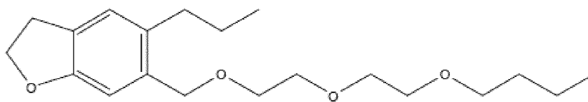
6-((2-(2-butoxyethoxy)ethoxy)methyl)-5-propyl-2,3-dihydrobenzofuran (Formula XII)
