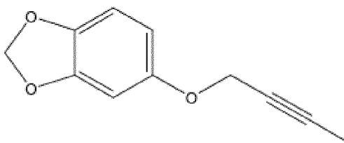
5-(but-2-ynoxy)benzo[d][1,3]dioxole (Formula XIV)
