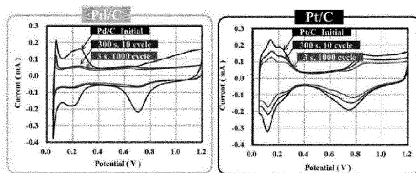
CV change of Pd/C core and Pt/C catalyst due to ADT
