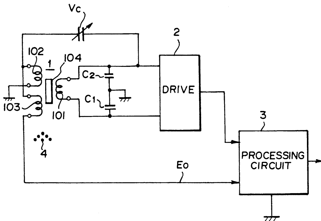
FIG. 4 (PRIOR ART)
