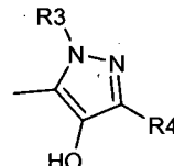
Formula (8c)
