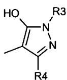
Formula (8a)
