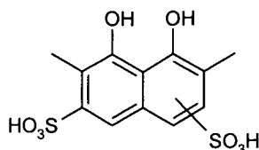
Formula (4);
