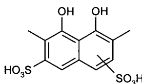
Formula (4);
