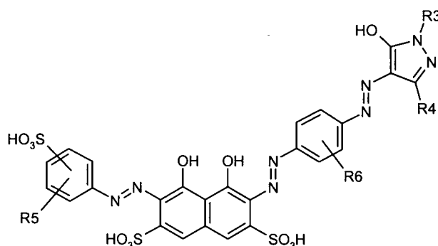
Formula (9)
