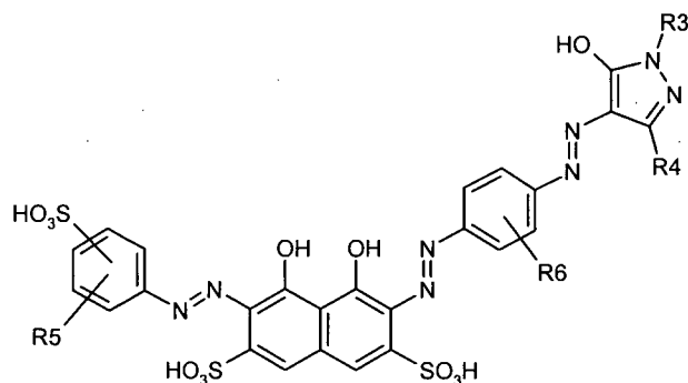
Formula (9)
