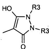
Formula (8b)
