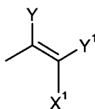
Formula (2)
