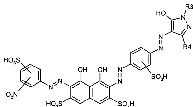
Formula (10).
