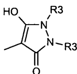
Formula (8b)
