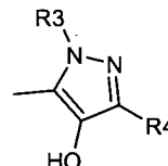
Formula (8c)
