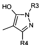
Formula (8a)
