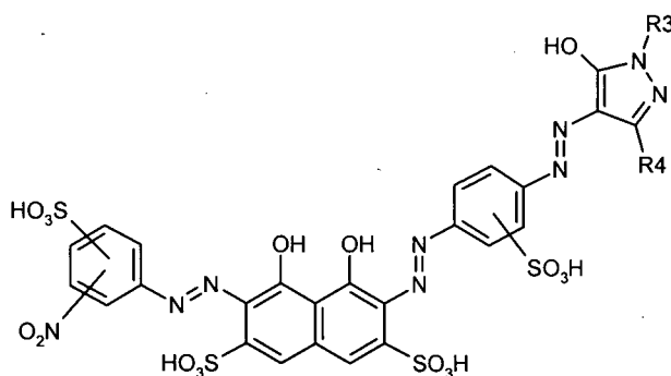
Formula (10)
