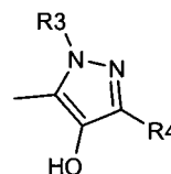
Formula (8c)
