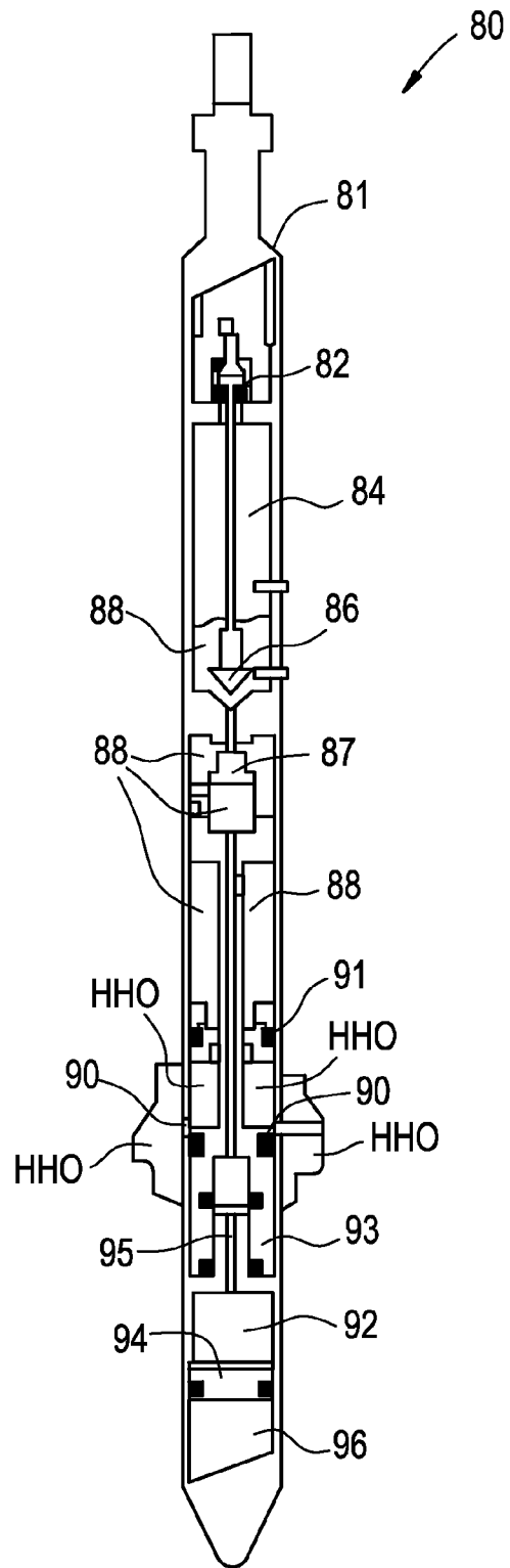
FIG. 5B (PRIOR ART)
