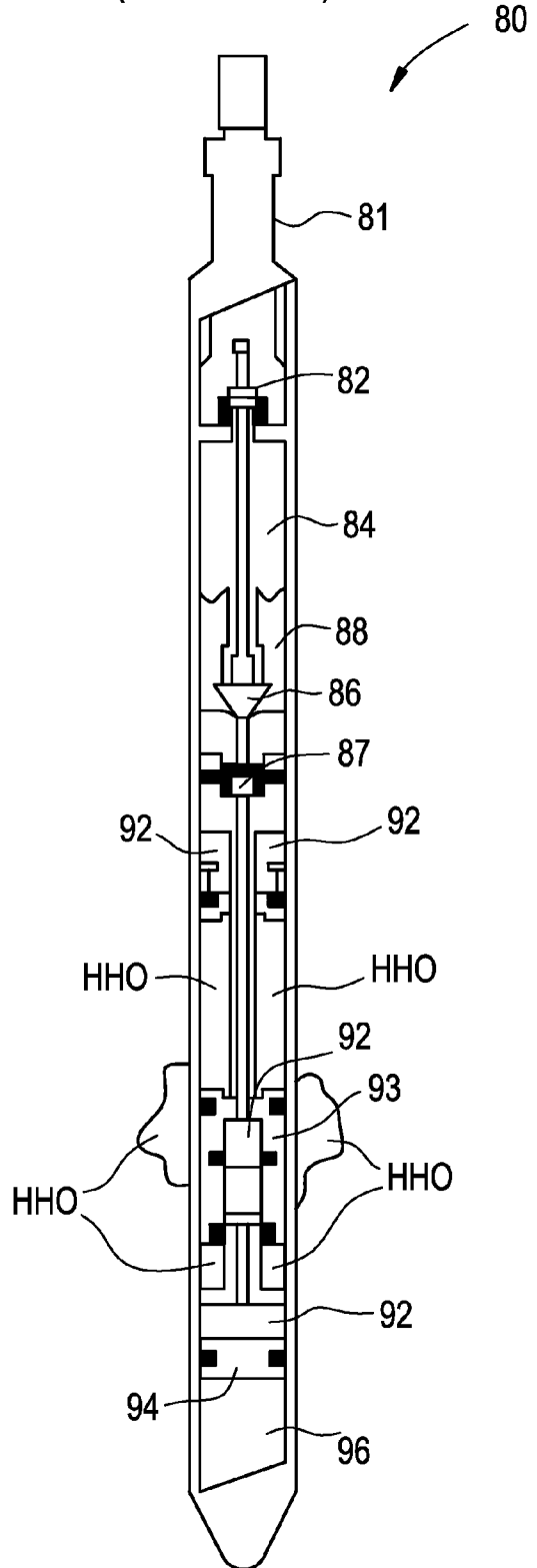
FIG. 5D (PRIOR ART)
