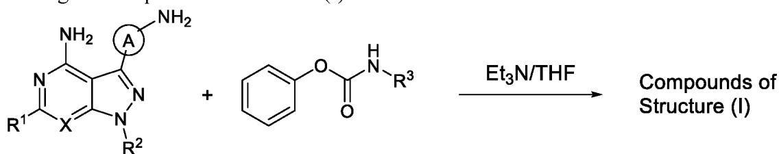
Intermediates B
