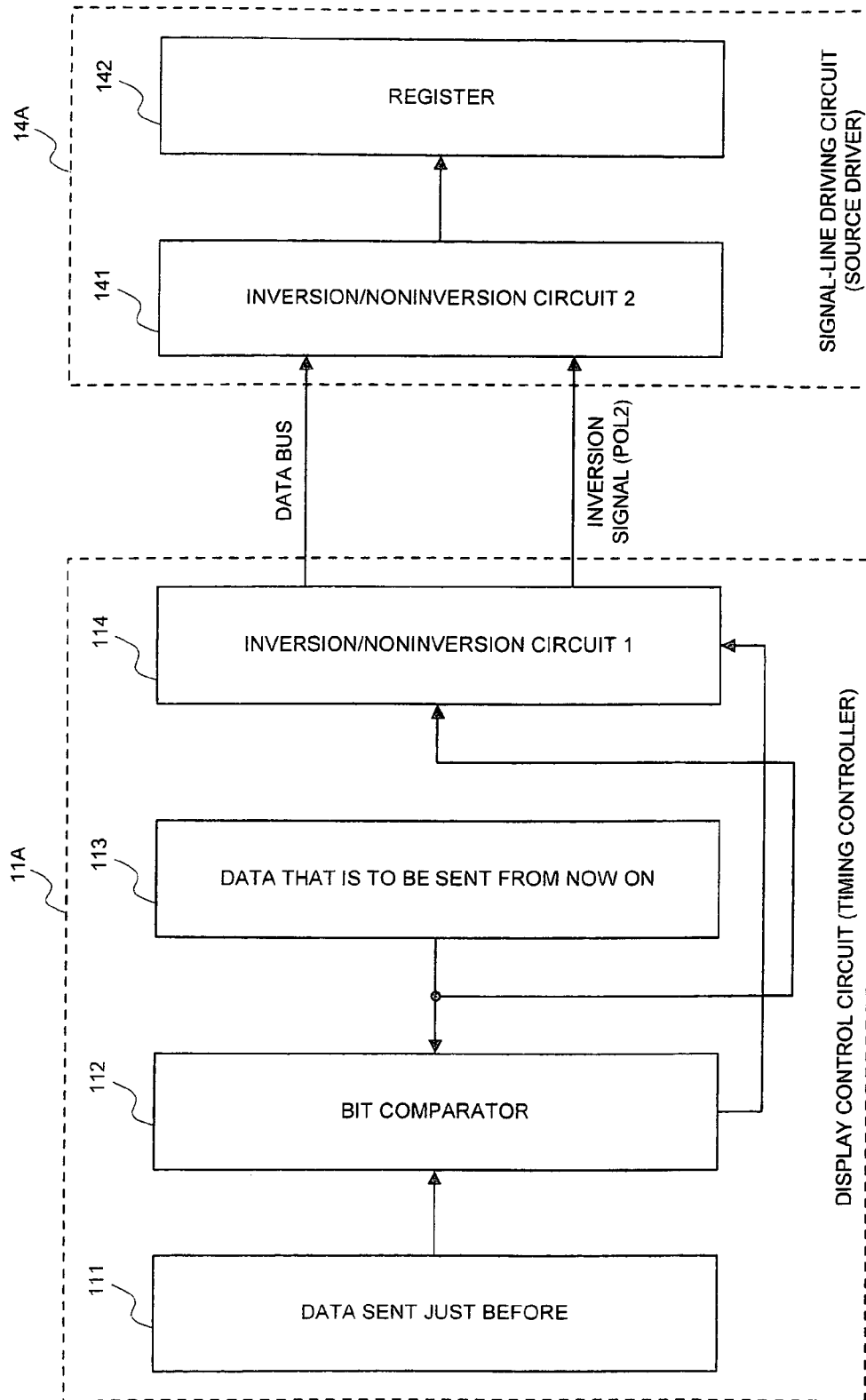
FIG. 9 PRIOR ART
