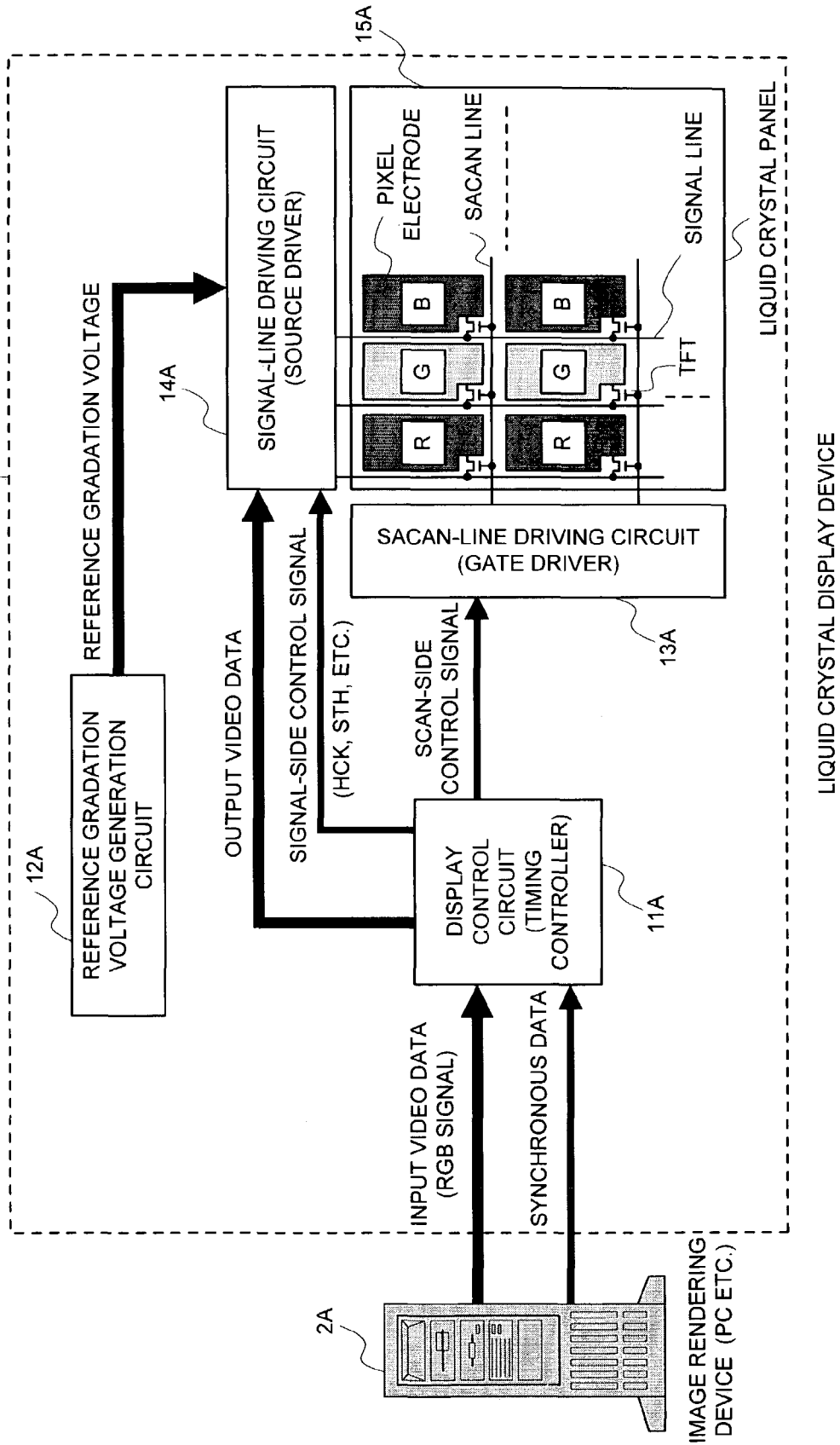
FIG. 8 PRIOR ART
