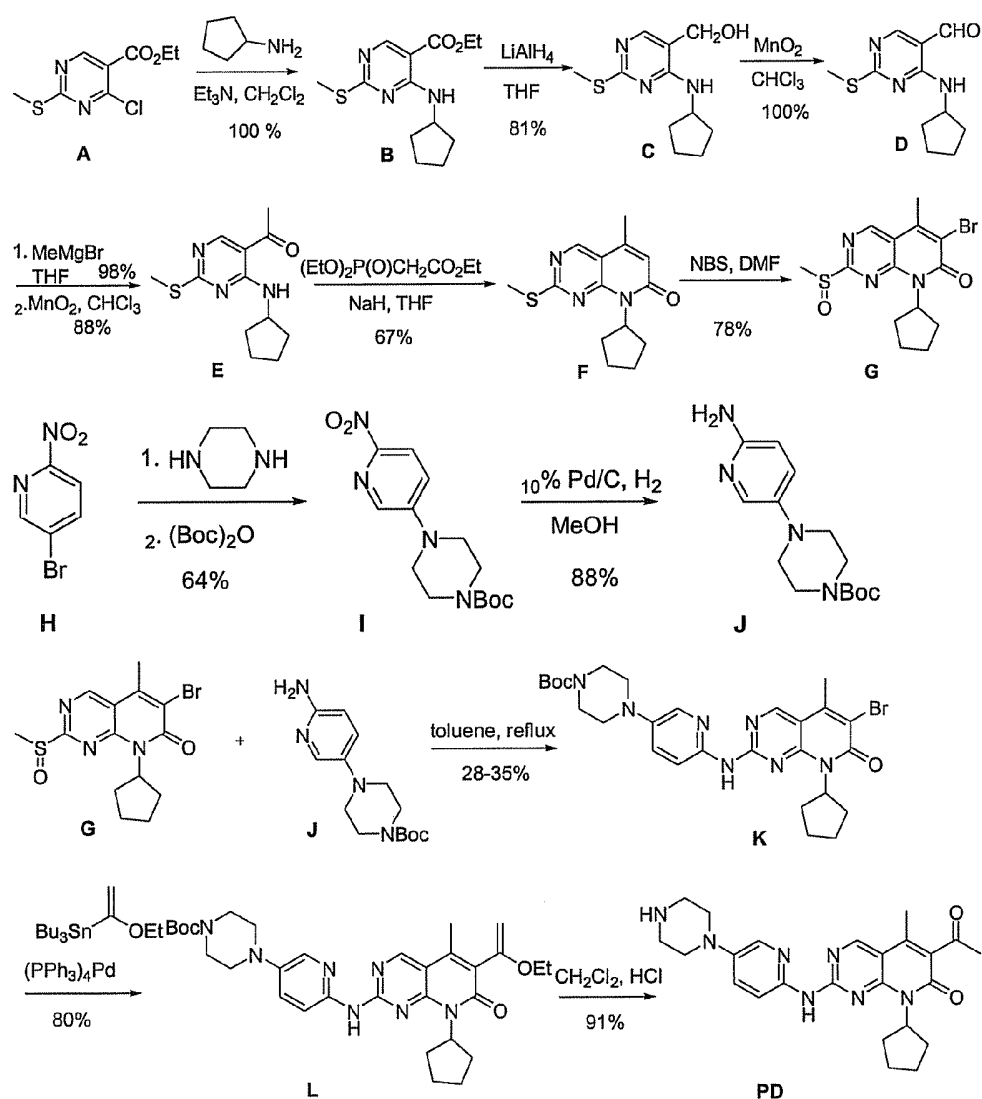
10 Scheme 1: Synthesis of PD.
