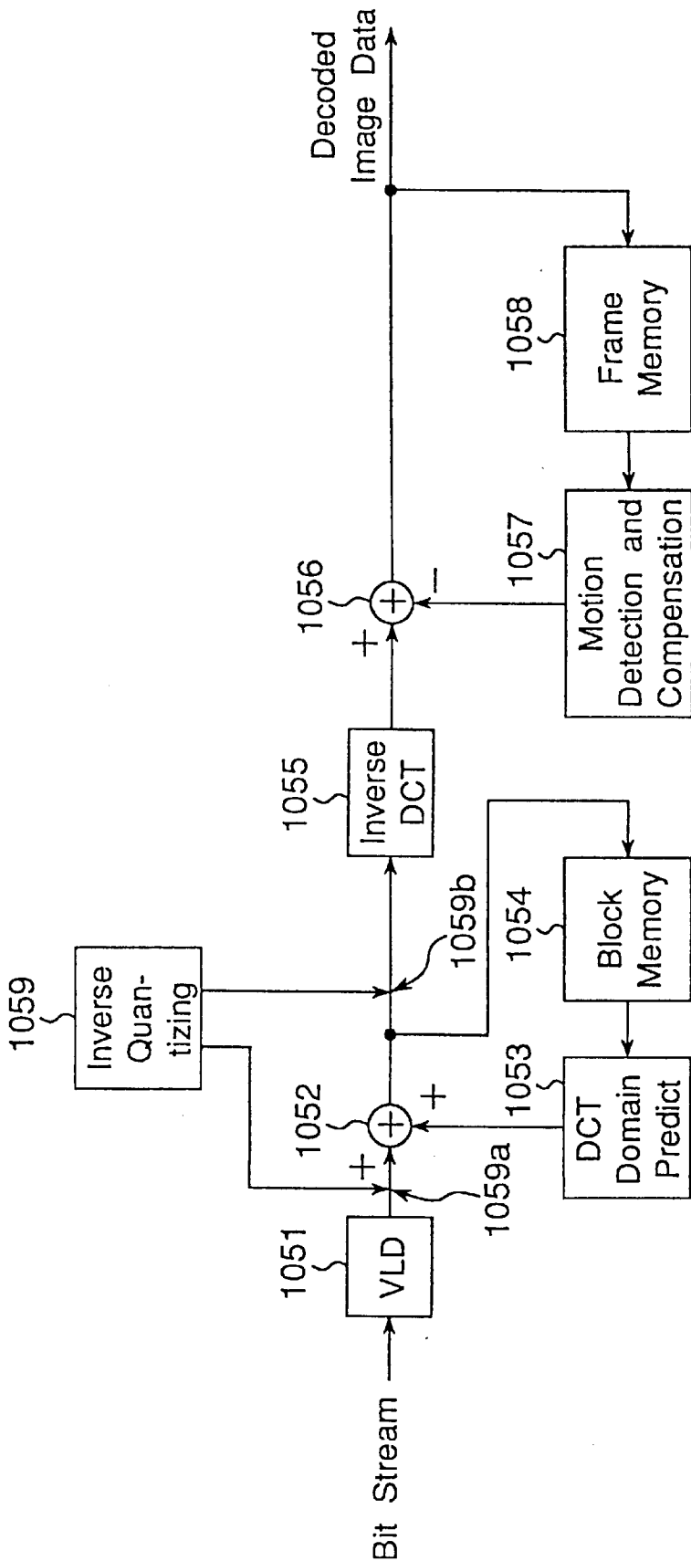
Fig.20 Seventh Preferred Embodiment Image Predictive Decoding Apparatus
