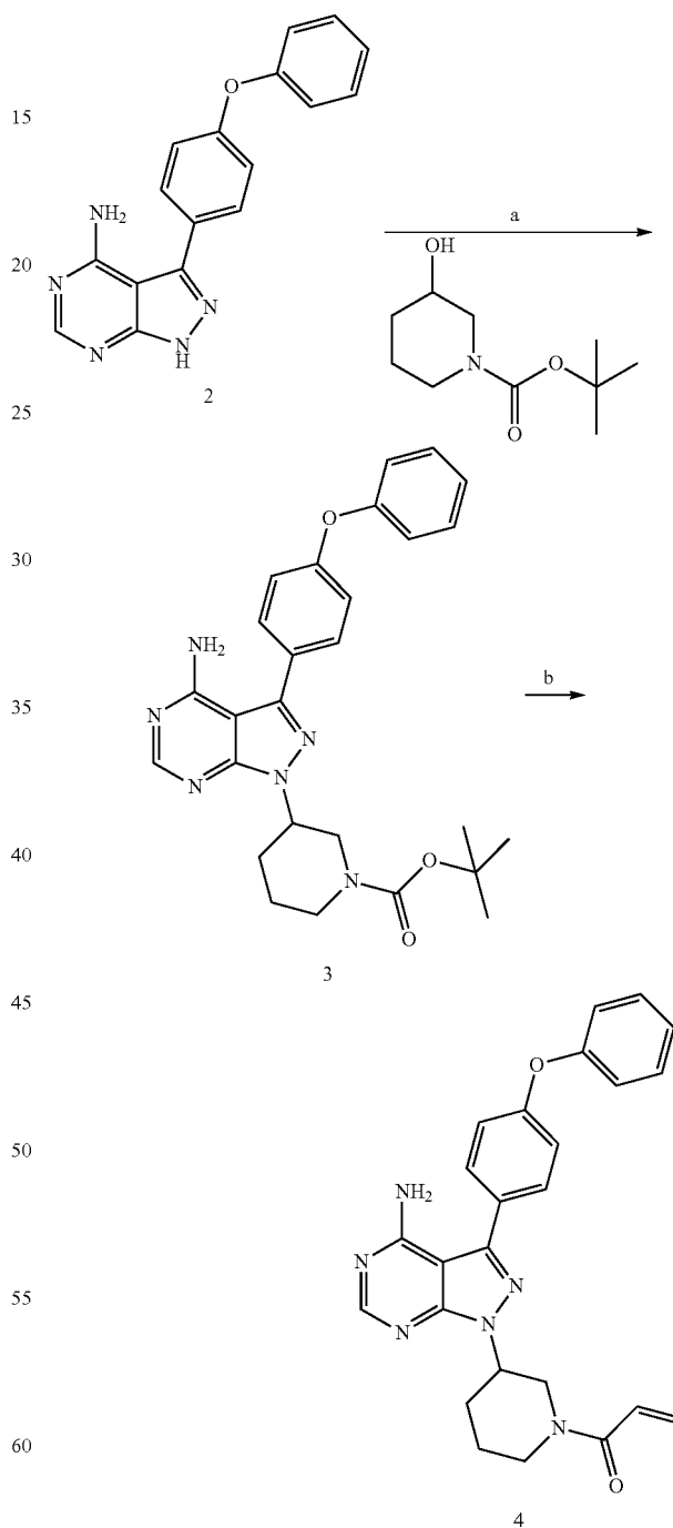
Scheme 1. Synthesis of compound 4;
