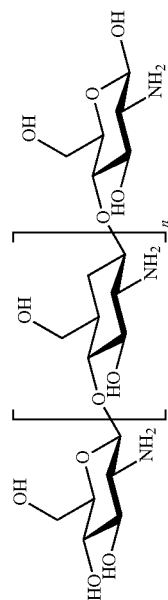
Chitosan
