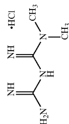
1,1-Dimethylbiguanide hydrochloride
