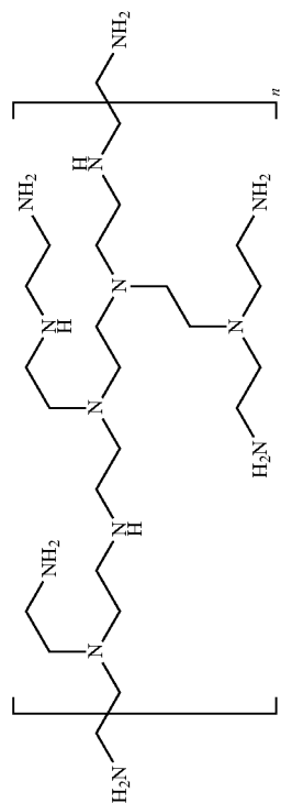
Branched Polyethylenimine
