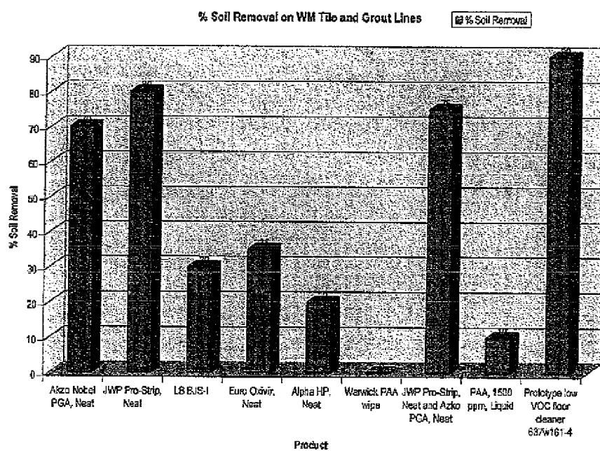
Figure 8. Summary of % soil removal of various cleaning products on Walmart restroom tile and grout. Testing performed on Thursday, August 10, 2006 in Racine Walmart.
