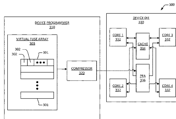
MICROPROCESSOR FUSE ARRAY COMPRESSION SYSTEM
