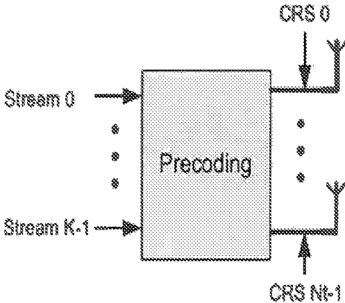
Figure 5 - Non-precoded cell-specific RS
