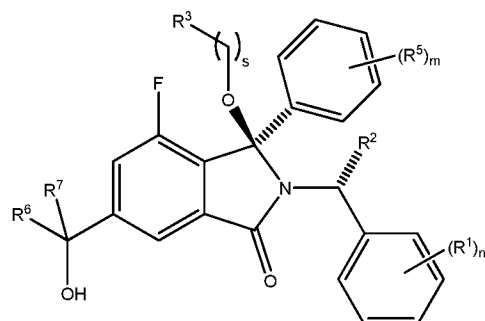
Diastereoisomer 1B
