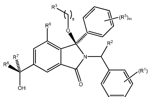
Diastereoisomer 2B
