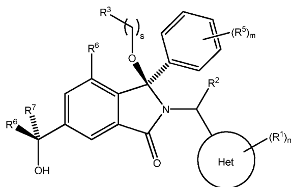
Diastereoisomer 2B
