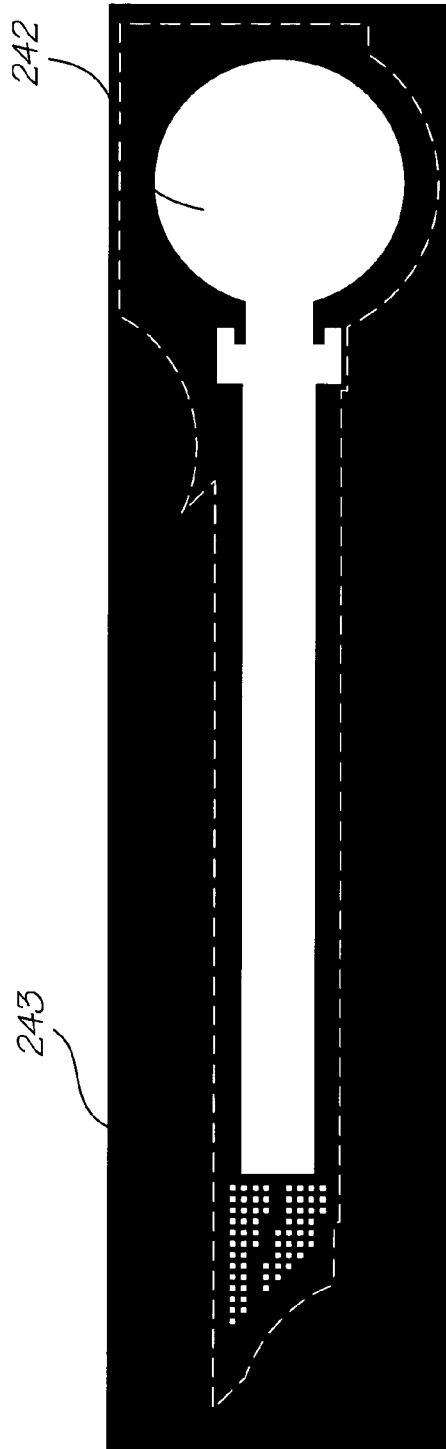
Via 3 / Passivation mask
