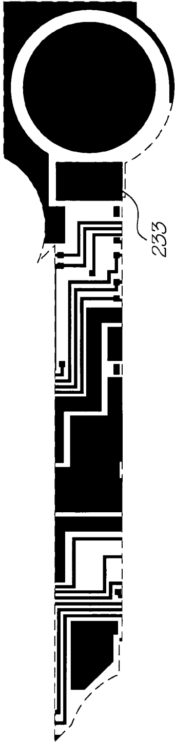
Metal 2 mask
