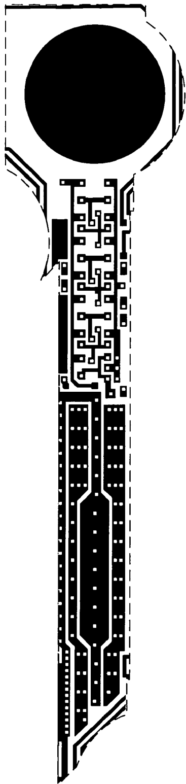
Metal 1 mask
