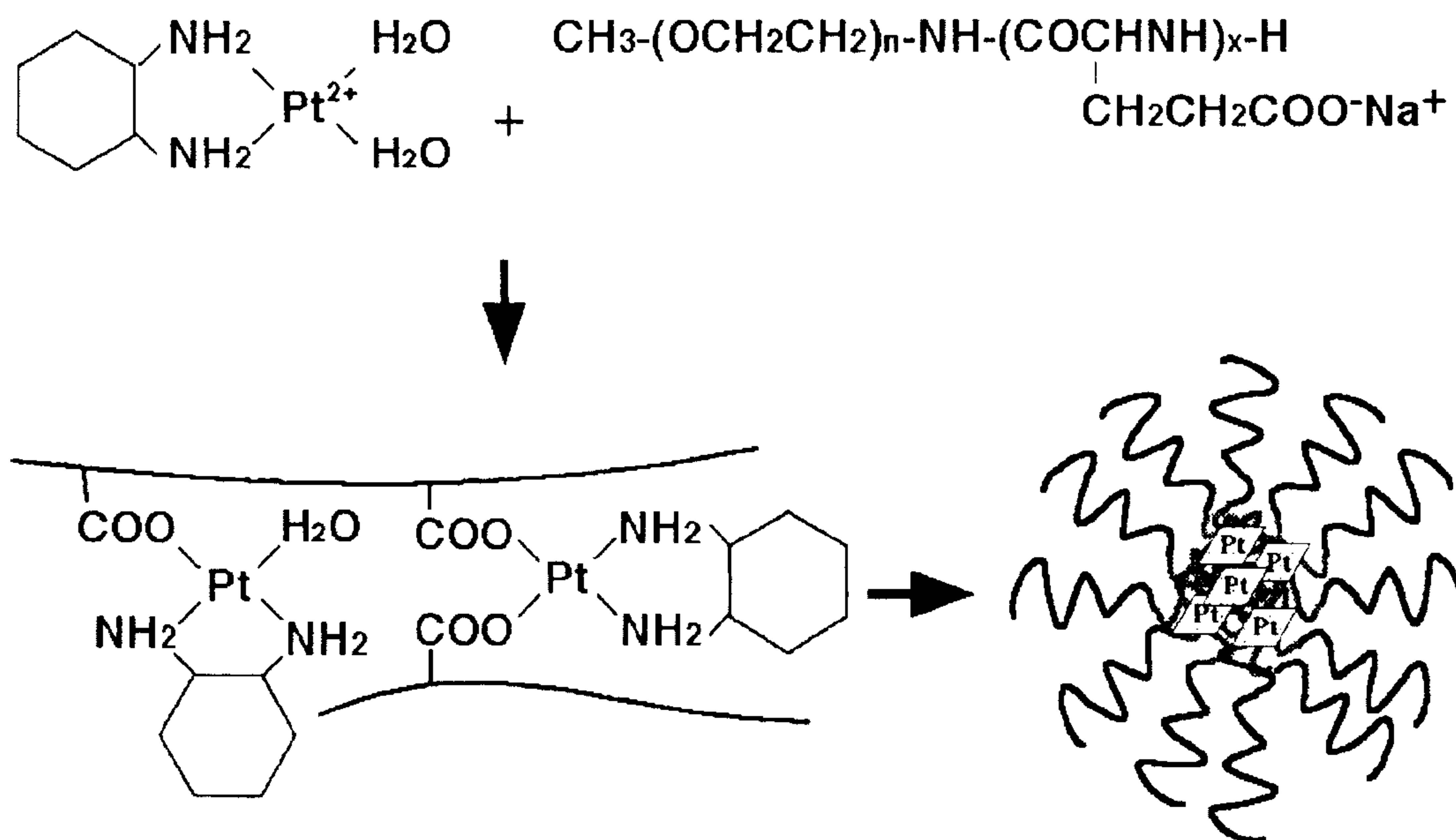
Drug encapsulated polymer micelle
