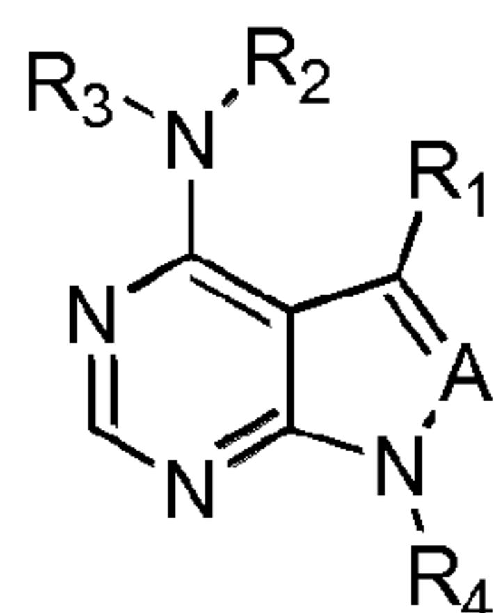
Formula (A);
