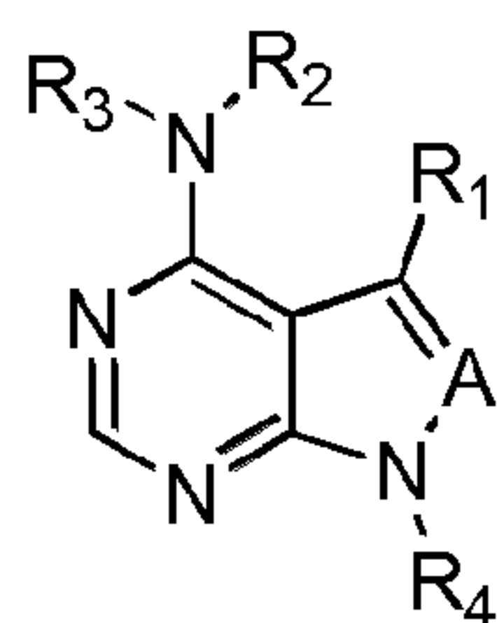
Formula (A)
