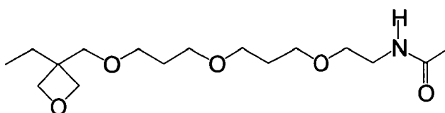
Compound (b-2)
