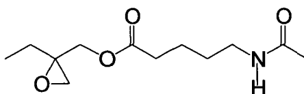
Compound (b-4)
