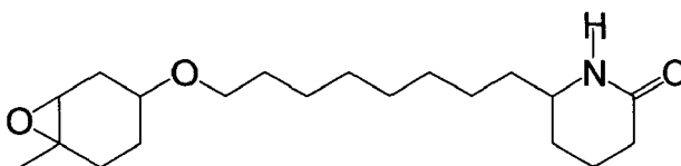
Compound (b-3)
