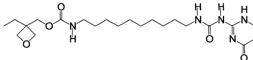
Compound (b-1)
