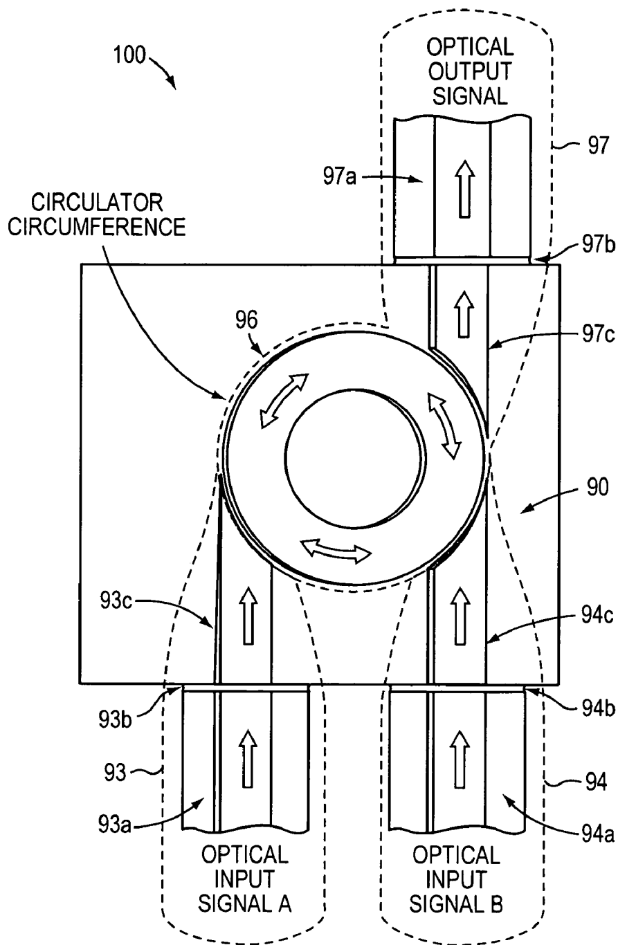
ALL-OPTICAL LOGICAL GATE USING CIRCULATOR WITHOUT SEPARATE COMBINING MEDIUM
