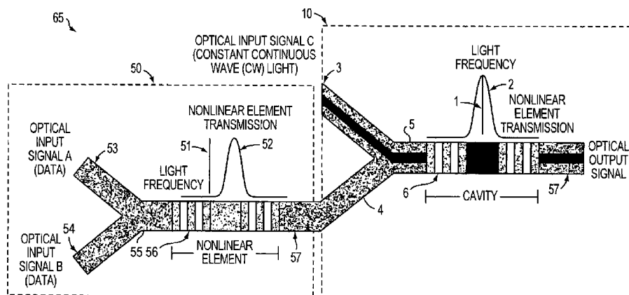
ALL-OPTICAL XNOR GATE WITH LOGIC LEVEL RESTORATION
