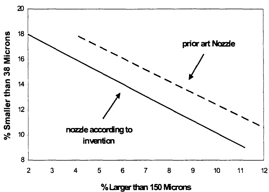
FIG. 5 The percentage product with less than 38 micron diameter at constant percentage of product greater than 150 micron.
