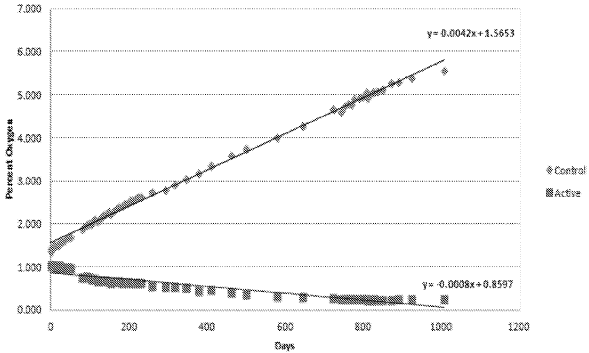
FIG. 1 Barrier Properties of Retorted Containers
