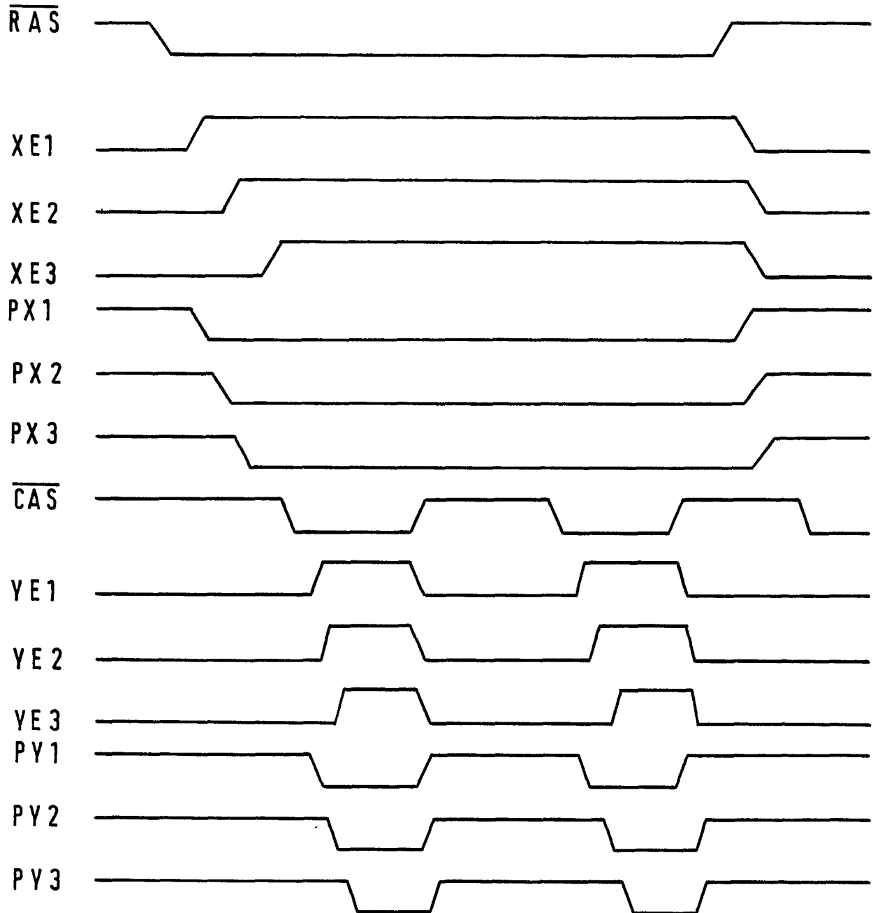
Fig.3 (Prior Art)
