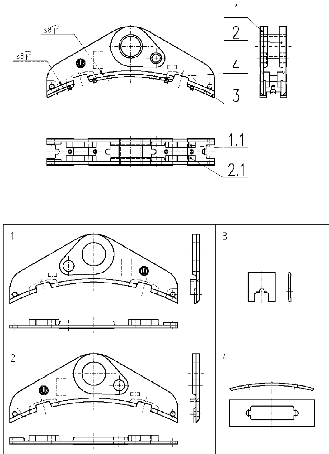
Picture 5: Double brake block holder and its drawn details 1, 2, 3 and 4.
