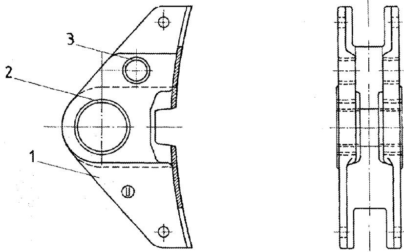
Picture 1: Brake block holder manufactured by forging in die or by casting into the form
