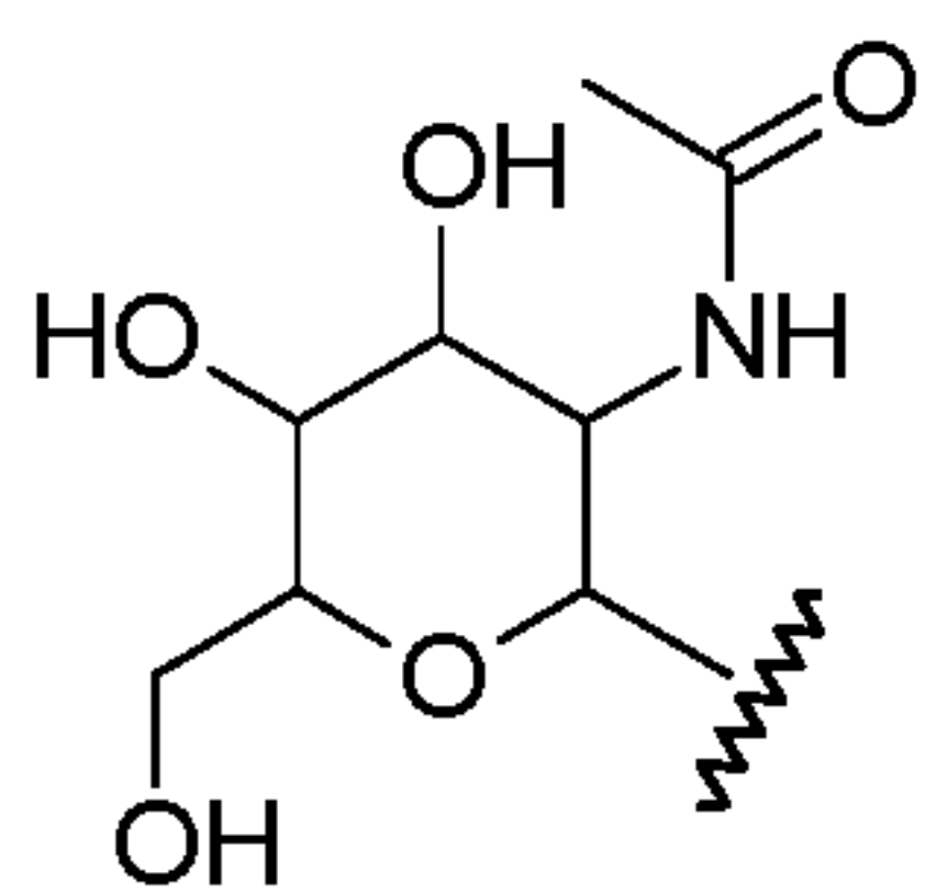
(N-acetyl-galactosamine).
