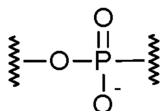
Phosphate group
