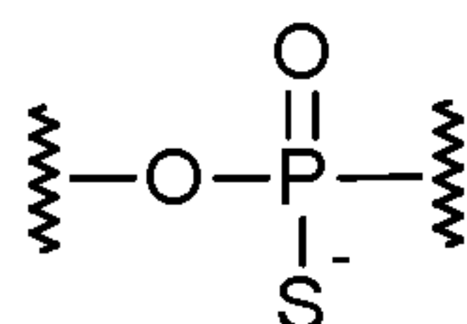
Phosphorothioate group
